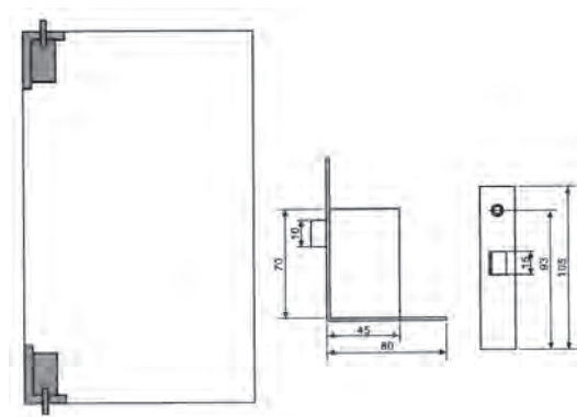
08-25745 Automatic Flush Bolt
